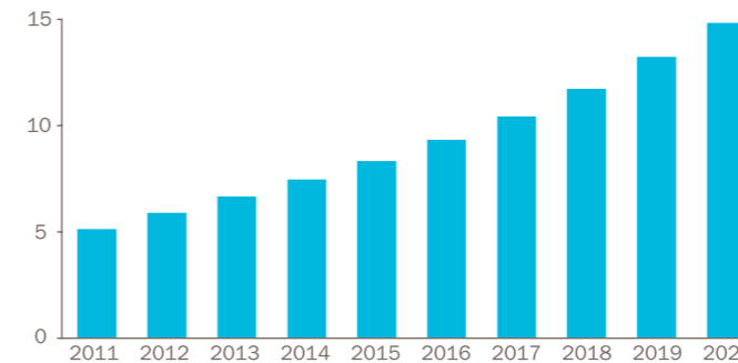
Total heat pump stock in 21 of EU's countries the last ten years (millions) 42
