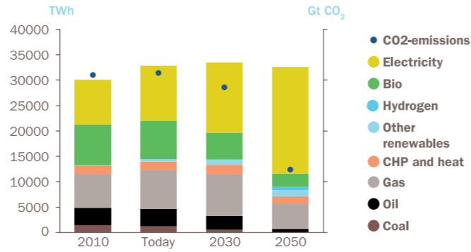
6 Global energy demand for buildings by energy carrier (TWh) (left) and total emissions for buildings (GtCO 2 ) (right).
