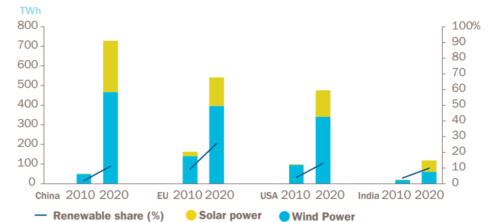
Wind and solar power production in China, USA, EU and India (TWh) and renewable share of total power production (%) 32
