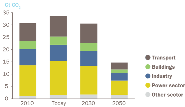
5 Global energy-related CO 2 emissions by sector (Gt CO 2 ).
