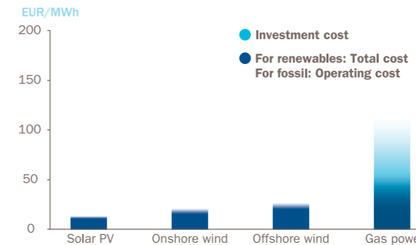
LCOE for different power producing technologies in Western-Europe in 2050
