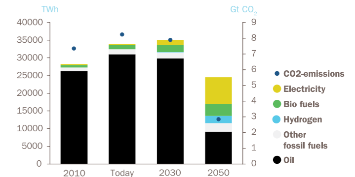
Global energy demand from the transport sector by energy carrier (TWh) (left) and total emissions for transport (Gt CO 2 ) (right)
