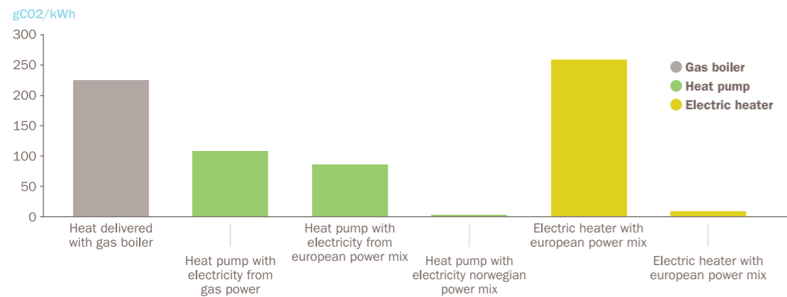
CO 2 -emissions from different heating solutions (gCO 2 /kWh)*
