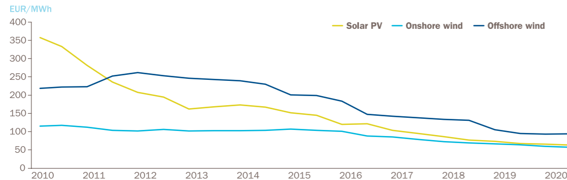
LCOE* for different renewable technologies 50
