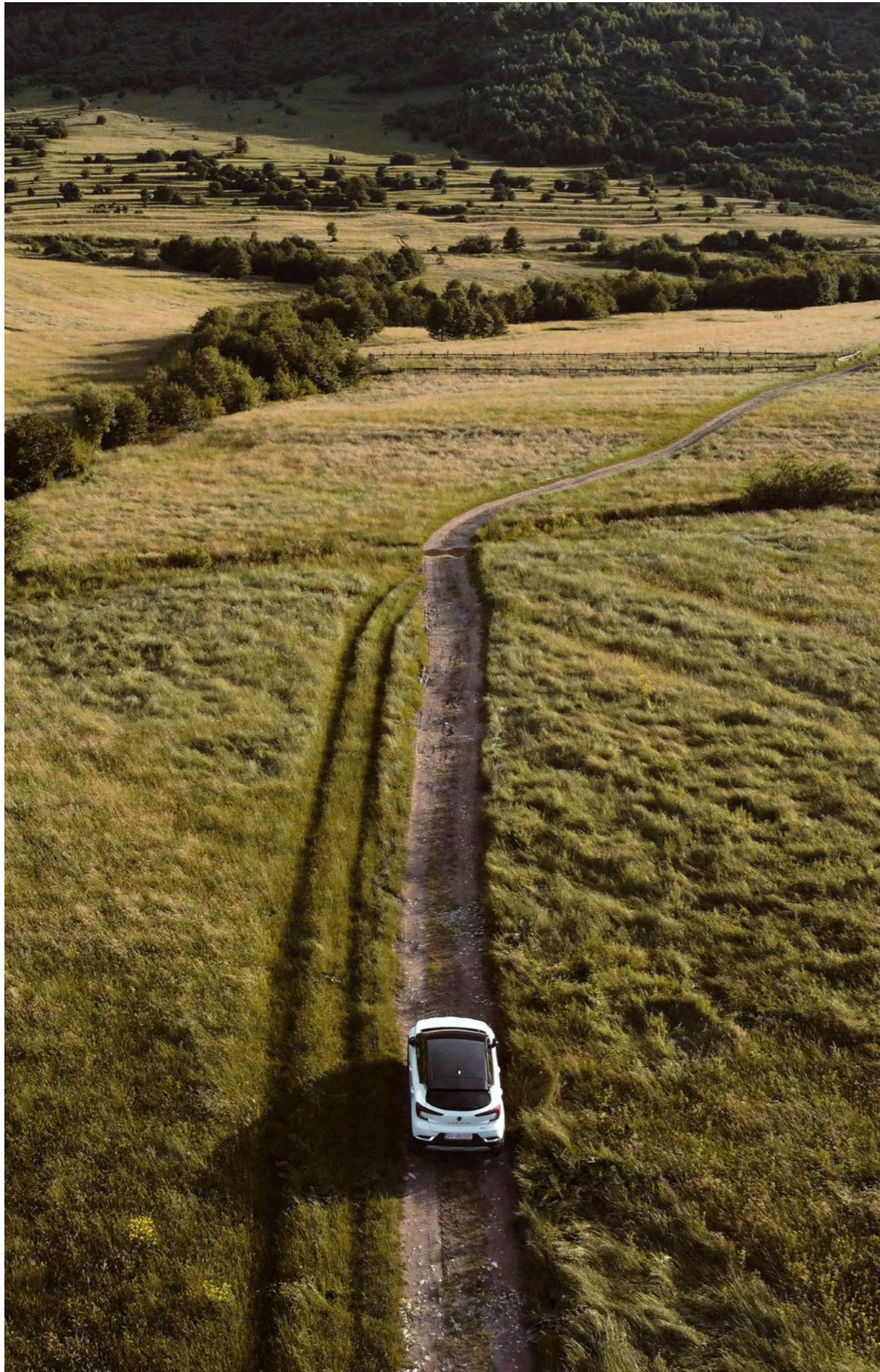
Recycling will be important for the demand for materials in batteries. However, the exponential growth in electric cars and energy storage means that only part of the demand growth will be met by recycling.
