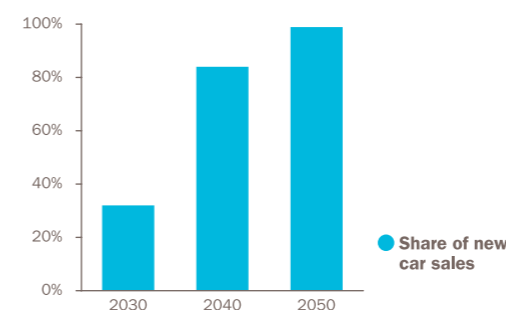
Emission-free share of new car sales globally
