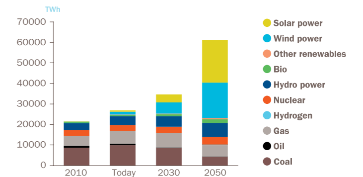
Power demand by energy carrier (TWh)
